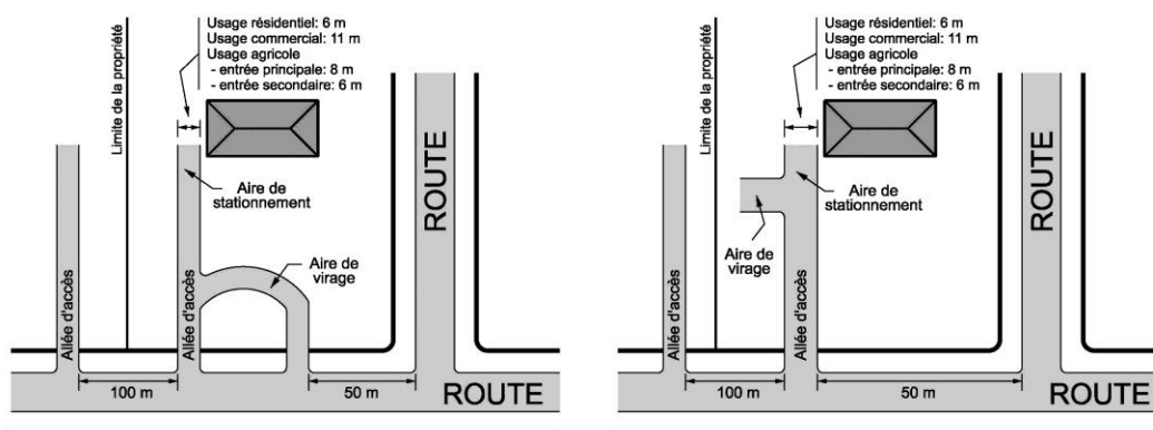
Croquis 11.3
